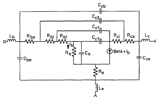
Fig. 4 HBT hybrid- \pi small signal equivalent circuit model
