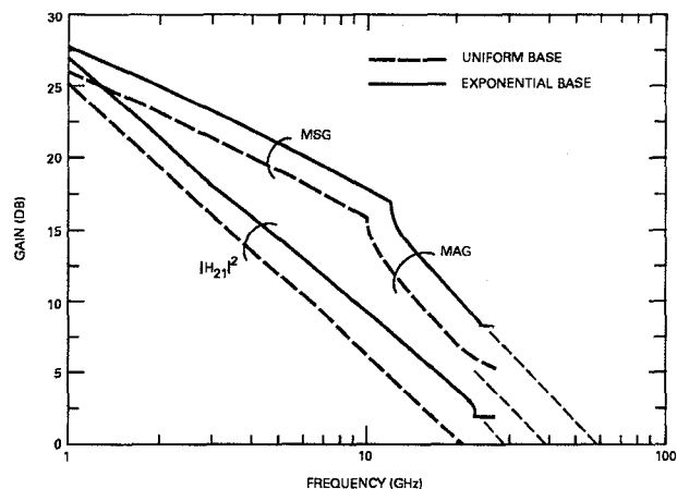
Fig. 3 Maximum stable/available gain and current gain (H21) vs.frequency for the uniform and exponentially graded base profiles
