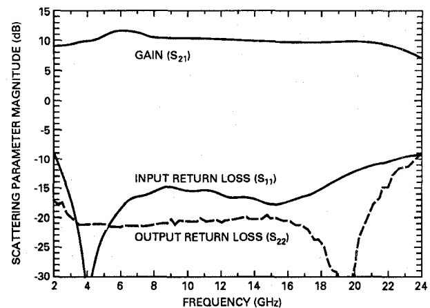
Fig. 7 Gain and input/output return-loss of the HBT matrix amplifier
